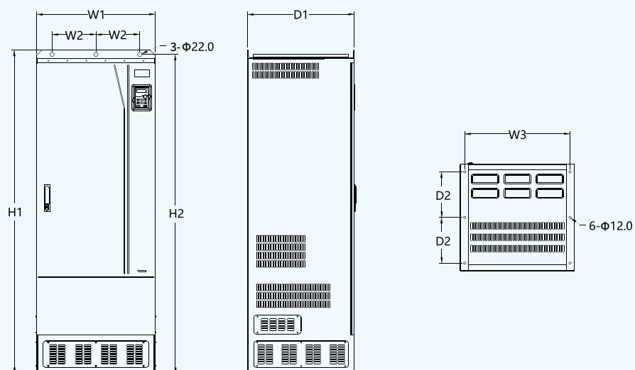
380V 355-500kW VFD floor installation diagram
