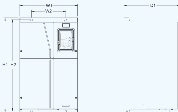
660V 22-132kW VFD wall-mounting diagram
