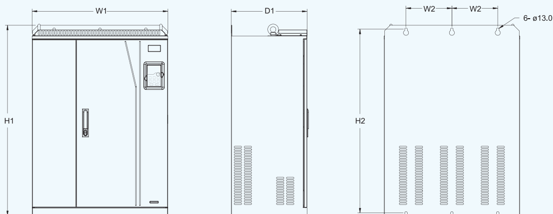
660V 250-355kW VFD wall-mounting diagram
