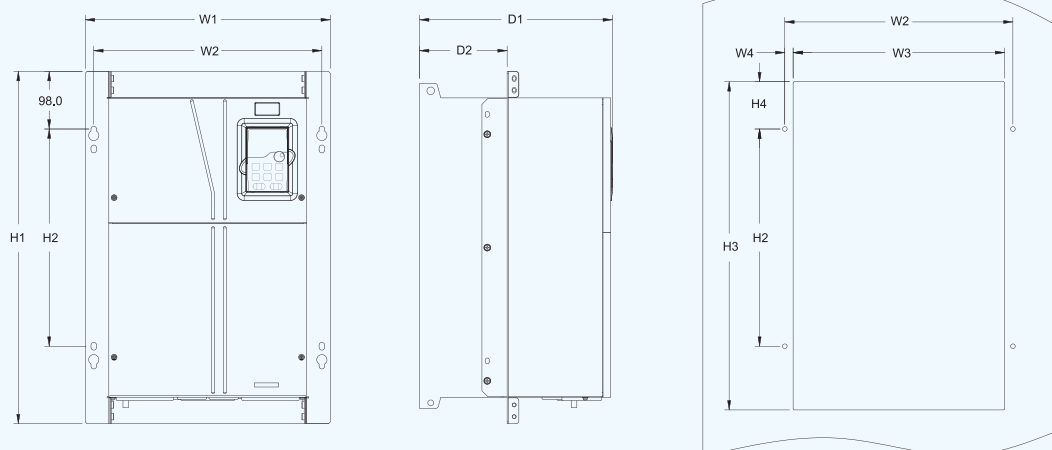
660V 22-132kW VFD flange installation diagram
