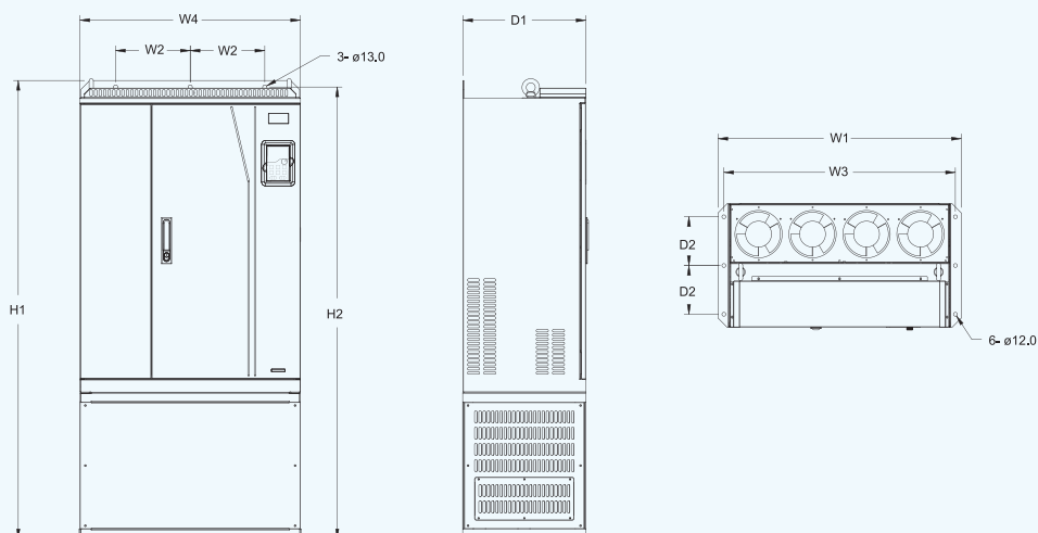
660V 250-355kW VFD floor installation diagram
