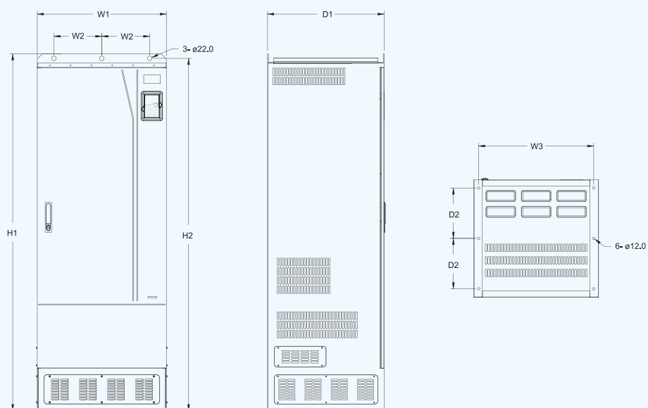
660V 400-630kW VFD floor installation diagram
