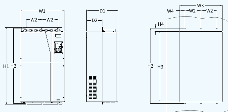
660V 160-220kW VFD flange installation diagram
