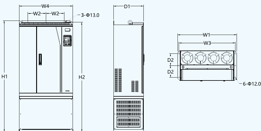
380V 220-315kW VFD floor installation diagram
