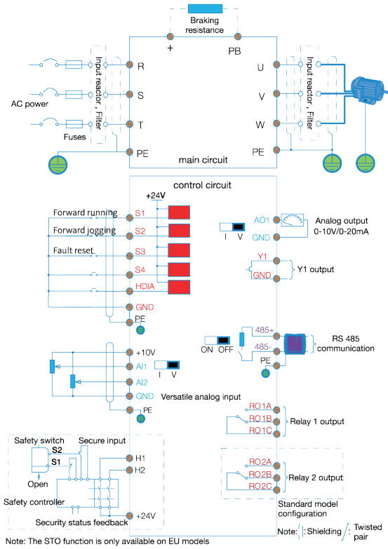
VFD wiring diagram
