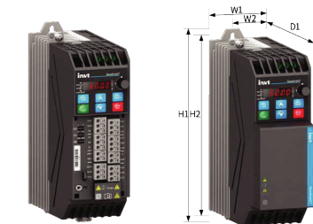
Uncovered outline drawing
