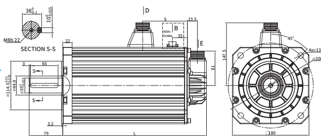
180 flange motor A type axes
