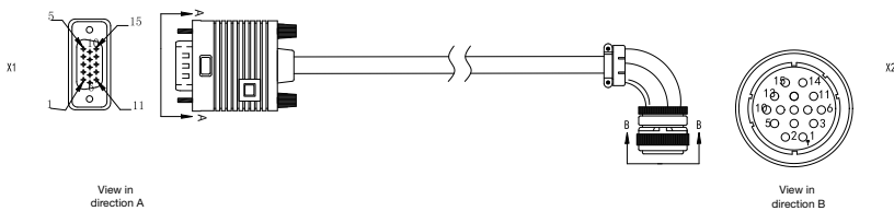
Cable for resolver encoder used by flange 200/263 motor
