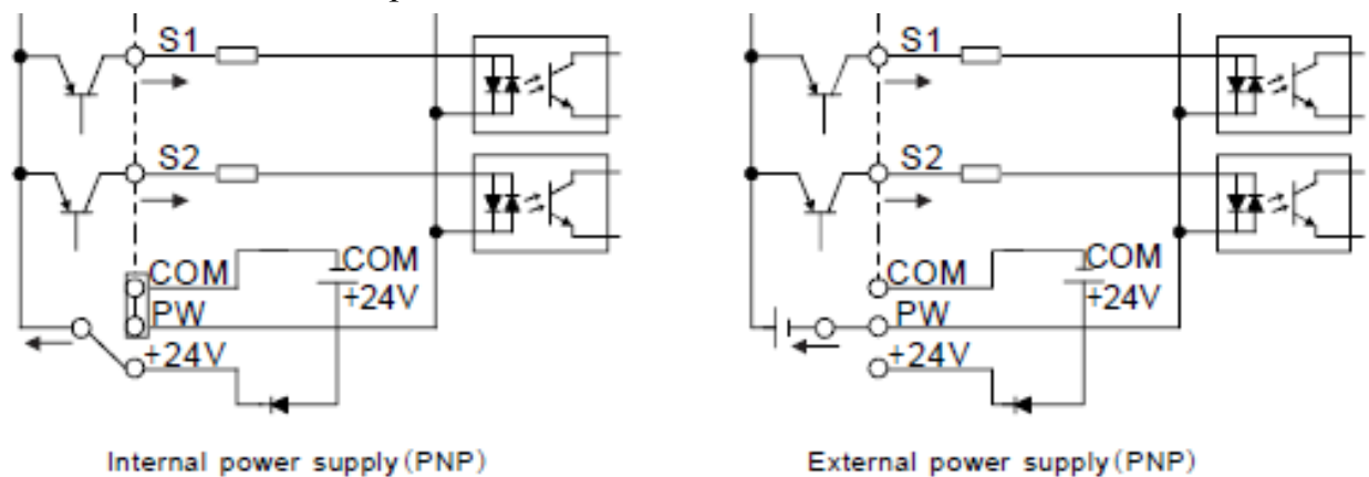
Fig 4-24 PNP modes
