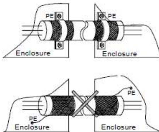
Fig 4-19 360 degree grounding technique
