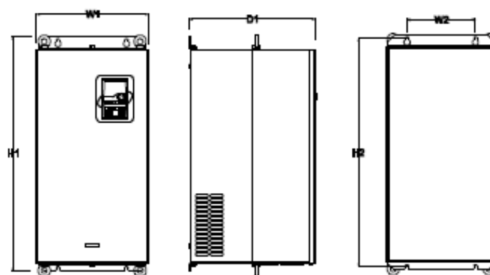
37-110kW wall mounting
