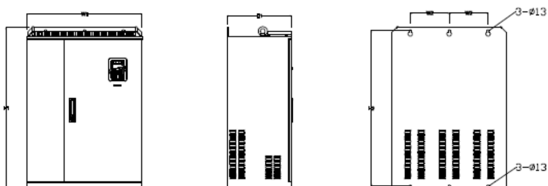
220-315kW wall mounting
