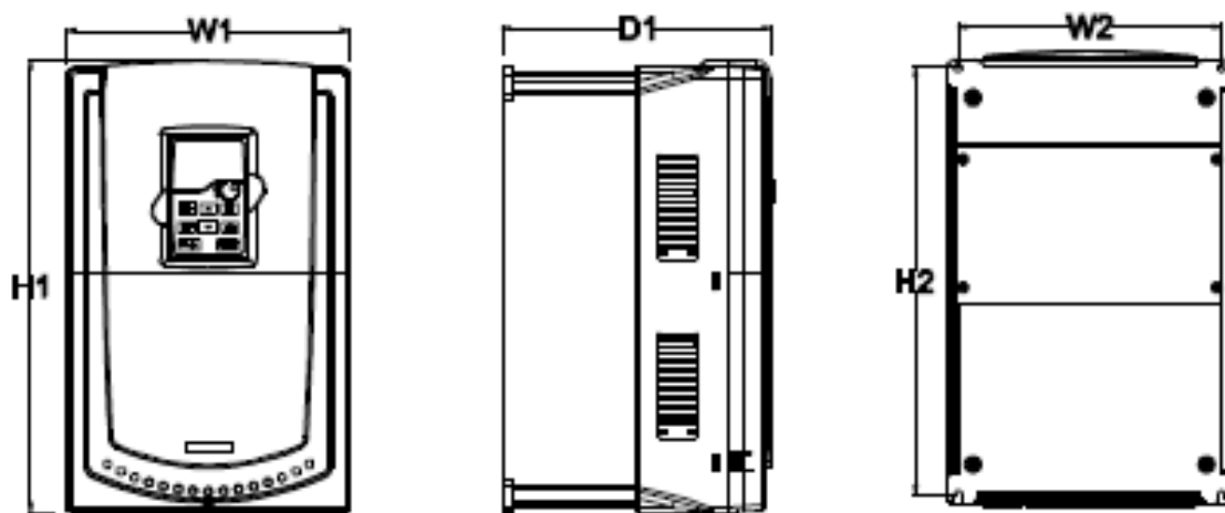
1.5-30kW wall mounting
