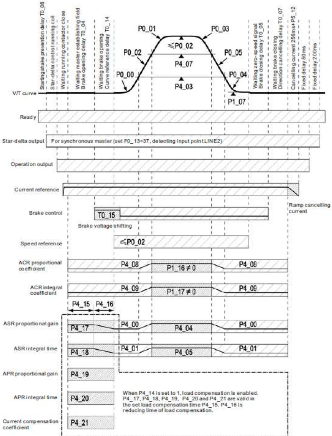
Fig 8-2 Sequence diagram
