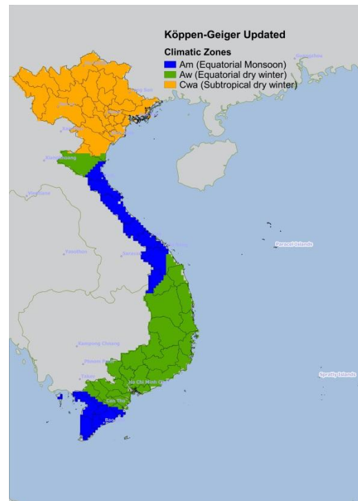
Fig. 1 Climatic zones in Vietnam according to Köppen-Geiger Climatic chart.
